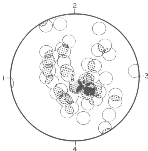
Fig. 27—Diagram of 50 compression axes derived from sets of e_1 twin lamellae in 50 calcite-cement crystals from an experimentally deformed calcite-cemented sandstone (from Friedman, Ref. 59, Fig. 16c). Specimen was shortened 9.2 per cent under 2-kb confining pressure at 300°C. Plane of the diagram is normal to the long axis of the deformed cylinder with the known position of \sigma_1 at the center of the diagram. Contours are at 2, 4, 6, and 8 per cent per 1 per cent area. The derived position of \sigma_1 is 10 to 15 degrees SE of the center.
